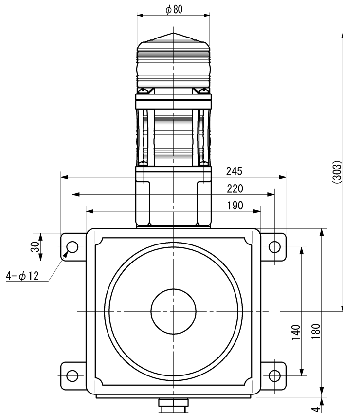
CABLE GLAND WITH SEAL PLUG 盲栓付き電線貫通金物
